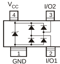
Device Schematic
