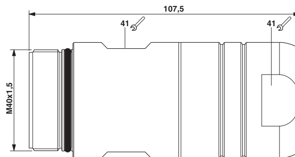
Dimensioned drawing
