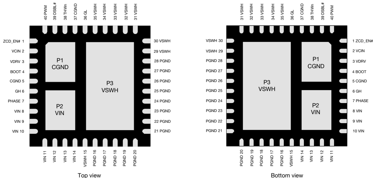
Fig. 2 - SiC783A Pin Configuration
