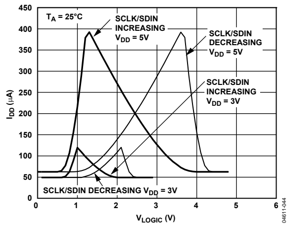
Figure 32. SCLK/SDIN vs. Logic Voltage
