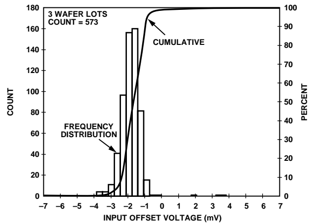
Figure 58. AD9632 Input Offset Voltage Distribution
