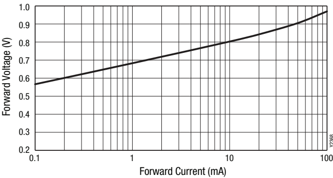
Figure 2. DC Characteristics
