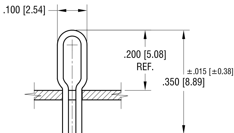
SHOWN AS INSTALLED INTO .067 [1.70] TO .078 [1.98] DIA. MOUNTING HOLE
