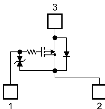
Fig. 7.1 Equivalent Circuit
