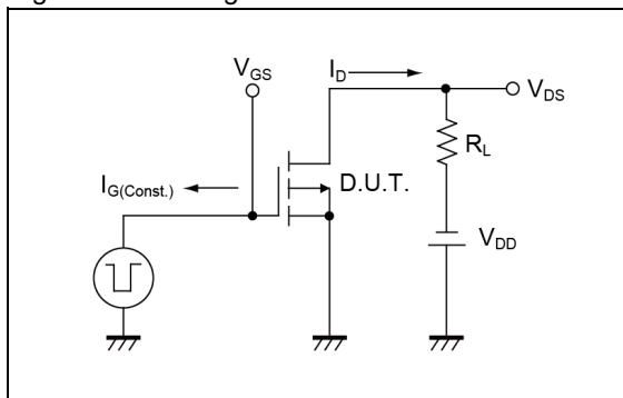
Fig.5-1 Gate Charge Measurement Circuit
