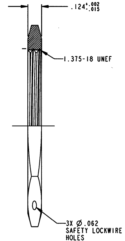
SECTION Z-Z
