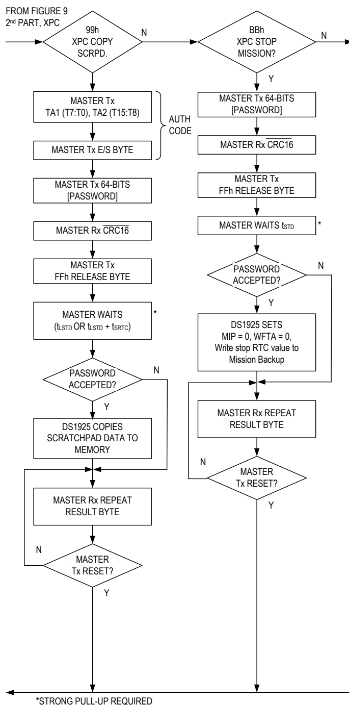
Figure 9c. Memory/Control Function Flowchart—XPC Subcommands Flowchart (continued)
