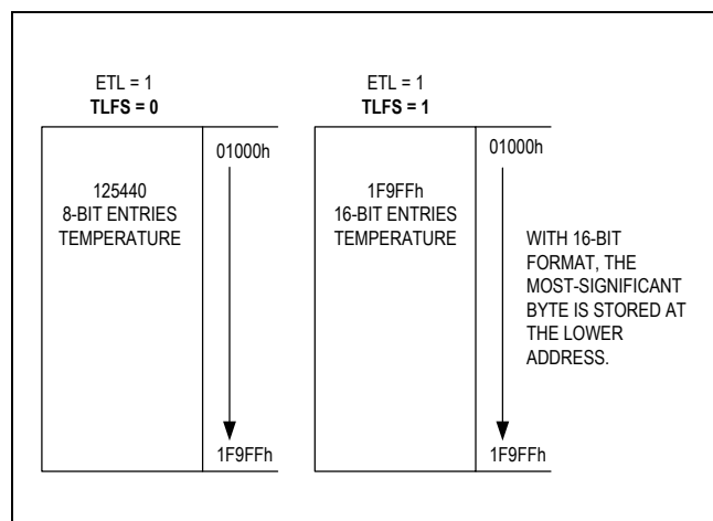
Figure 7. Temperature Logging
