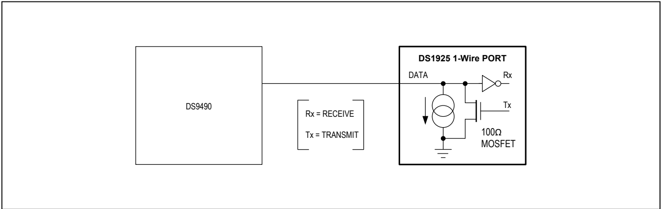
Figure 10. Hardware Configuration
