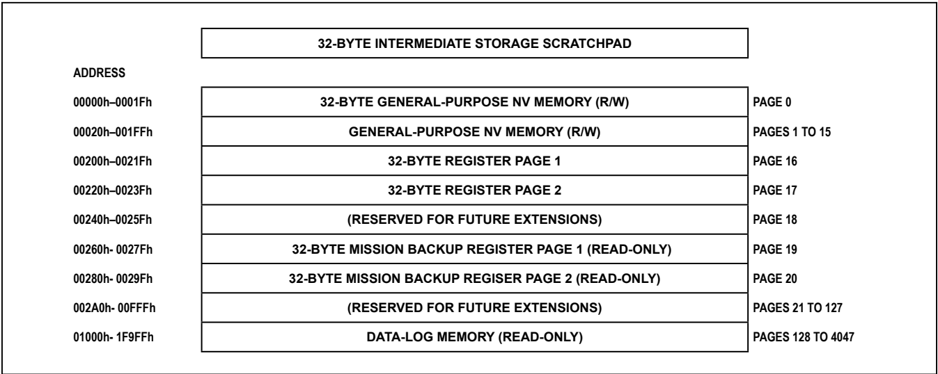
Figure 5. Memory Map
