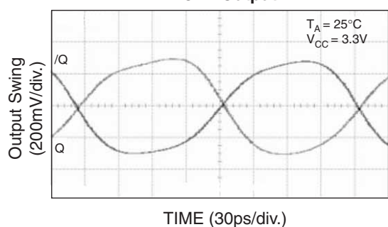
4GHz Output
