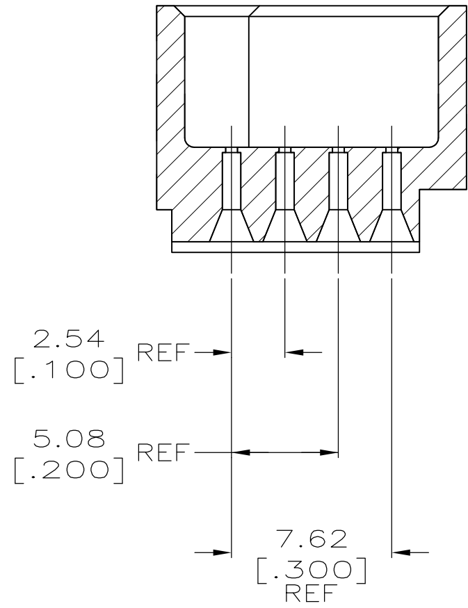
SECTION S-S
