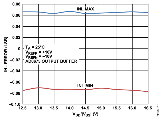
Figure 15. Integral Nonlinearity Error vs. Supply Voltage, \pm 10 V Span
