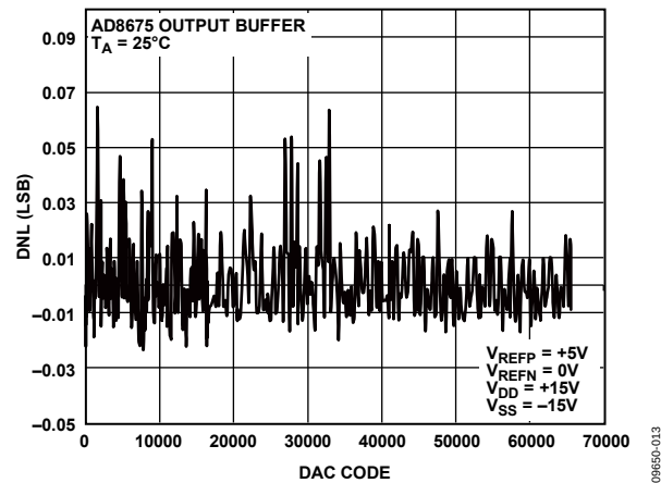
Figure 12. Differential Nonlinearity Error vs. DAC Code, 5 V Span, \times 2 Gain Mode
