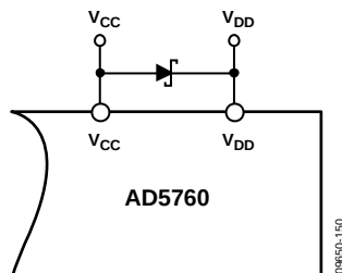
Figure 50. Schottky Diode Connection
