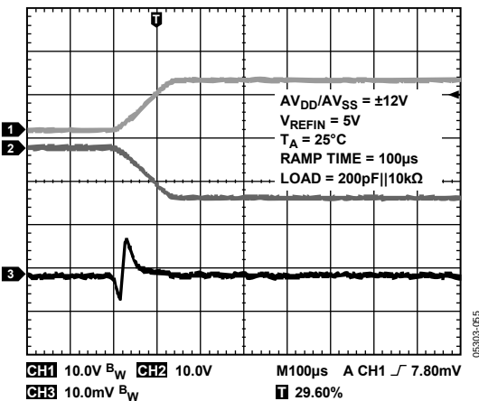
Figure 30. V_{OUT} vs. AV_{DD}/AV_{SS} on Power-Up
