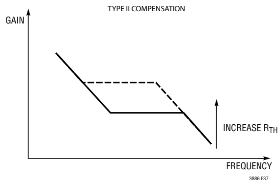
Figure 37. R_{I_{TH}} Adjust
