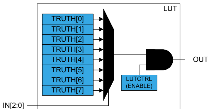
Figure 40-2. Truth Table Output Value Selection
