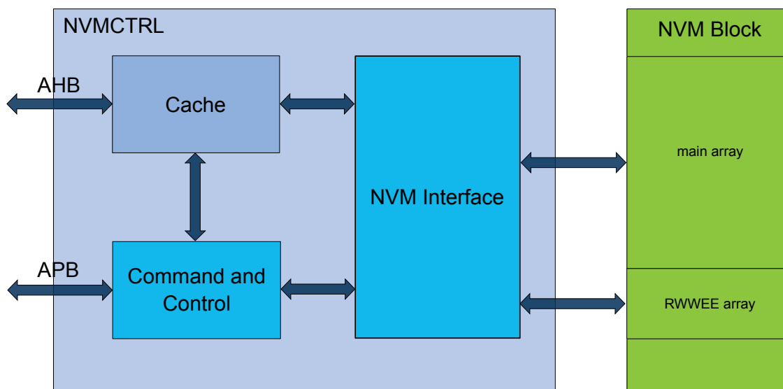
Figure 28-1. Block Diagram
