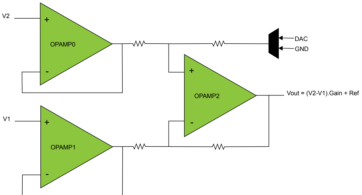
Figure 41-8. Instrumentation amplifier
