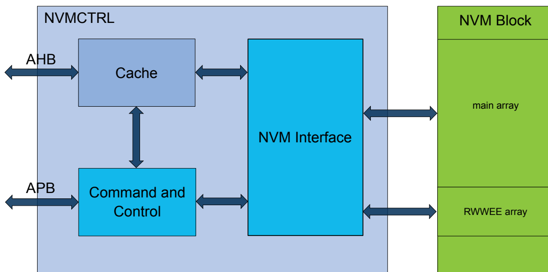
Figure 28-1. Block Diagram
