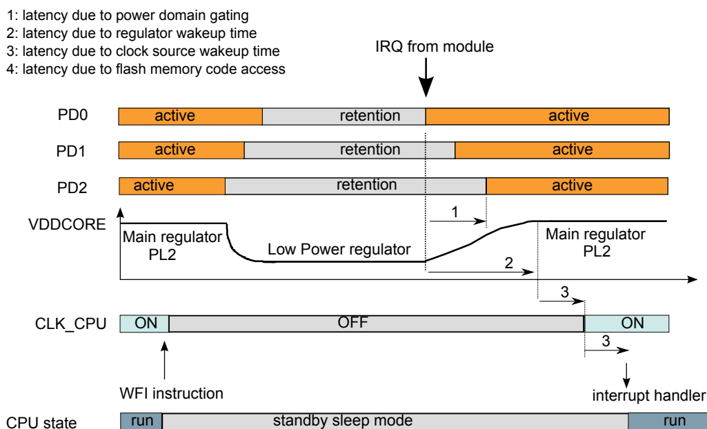
Figure 20-5. Total Wake-up Time from Standby Sleep Mode
