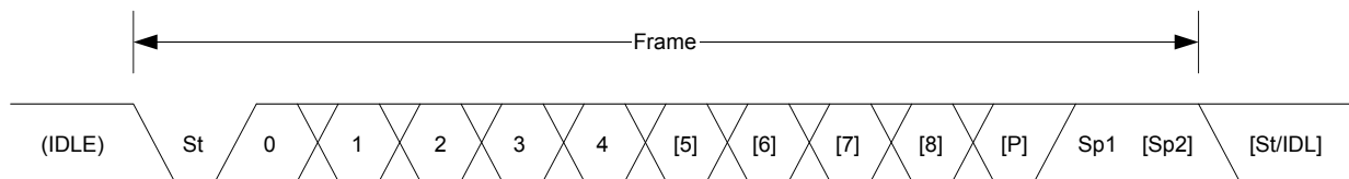
Figure 32-2. Frame Formats
