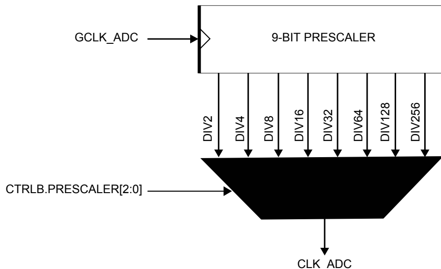
Figure 42-2. ADC Prescaler
