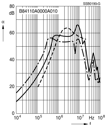
Filters for 4 A
