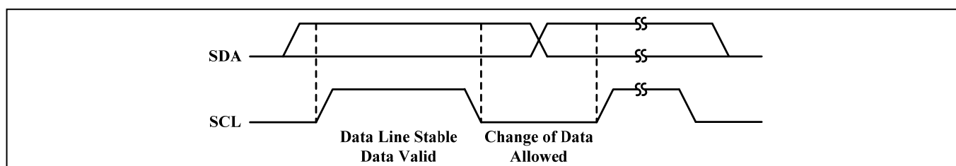
Figure 4 Bit Transfer
