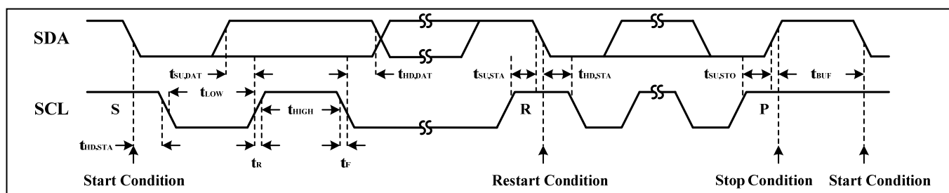
Figure 3 Interface Timing
