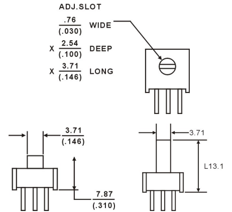
TSR-3386(STYLE)-EY5-(RESISTANCE CODE)
