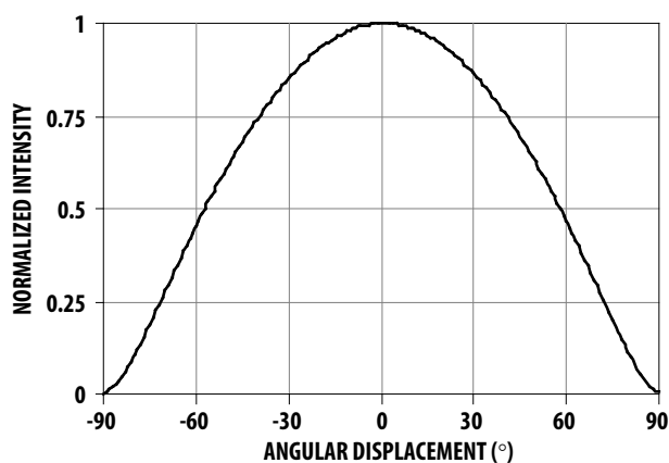
Figure 4: Radiation Pattern
