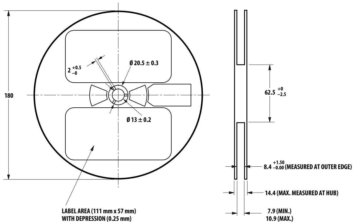
Figure 10: Reel Dimensions (Unit: mm)
