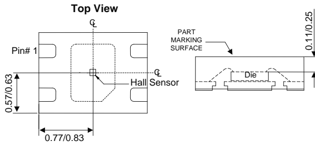
Sensor Location
