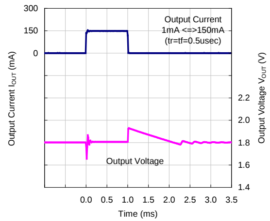
VR=1.8V, C_{OUT}=10\mu\text{F}
