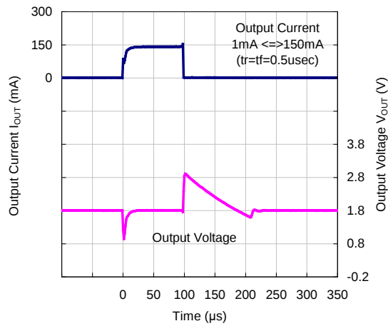
VR=1.8V, C_{OUT}=0.1\mu\text{F}
