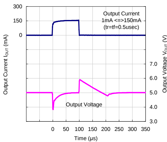
VR=5.0V, C_{OUT}=0.1\mu\text{F}
