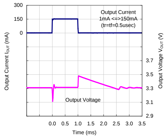
VR=3.3V, C_{OUT}=10\mu\text{F}
