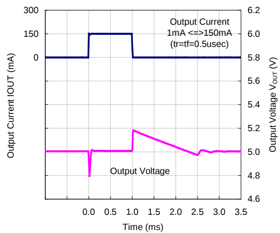
VR=5.0V, C_{OUT}=10\mu\text{F}
