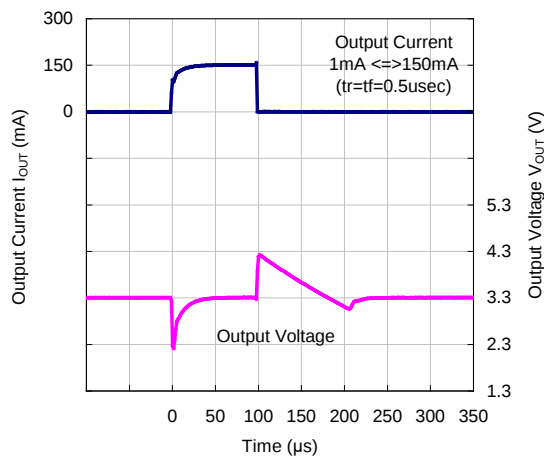
VR=3.3V, C_{OUT}=0.1\mu\text{F}
