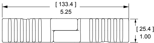
Mated Length
