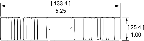
Mated Length
