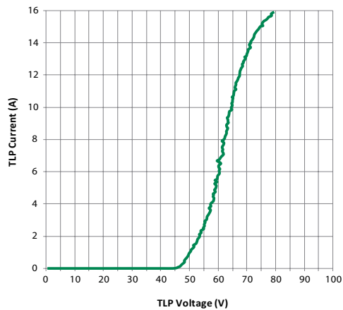
SPHV36-C Transmission Line Pulsing(TLP) Plot
