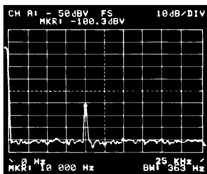
Figure 16. Multiplier Feedthrough
