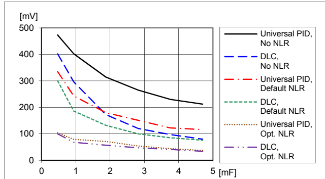
Load transient peak voltage deviation vs. external capacitance. Step (12.5-37.5-12.5 A). Parallel coupling of capacitors with 470 \mu F /10 m \Omega , T_{P1} = +25^\circ C . V_I = 12 V , V_O = 1.0 V , f_{sw} = 320 kHz , di/dt = 2 A/\mu s
