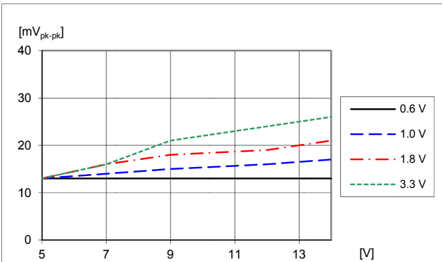
Output voltage ripple V_{pk-pk} at: T_{P1} = +25\text{ }^\circ\text{C} , C_O = 470\text{ }\mu\text{F}/10\text{ m}\Omega , I_O = 40\text{ A} .
