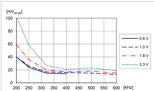
Output voltage ripple V_{pk-pk} at: T_{P1} = +25\text{ }^\circ\text{C} , V_I = 12\text{ V} , C_O = 470\text{ }\mu\text{F}/10\text{ m}\Omega , I_O = 40\text{ A} . Default configuration except changed frequency.
