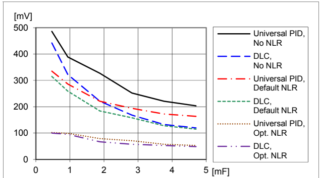
Load transient peak voltage deviation vs. external capacitance. Step (12.5-37.5-12.5 A), Parallel coupling of capacitors with 470 \mu F /10 m \Omega , T_{P1} = +25^\circ C . V_I = 12 V , V_O = 3.3 V , f_{sw} = 320 kHz , di/dt = 2 A/\mu s
