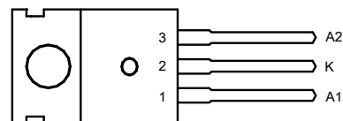
TO-220-3 (2)
