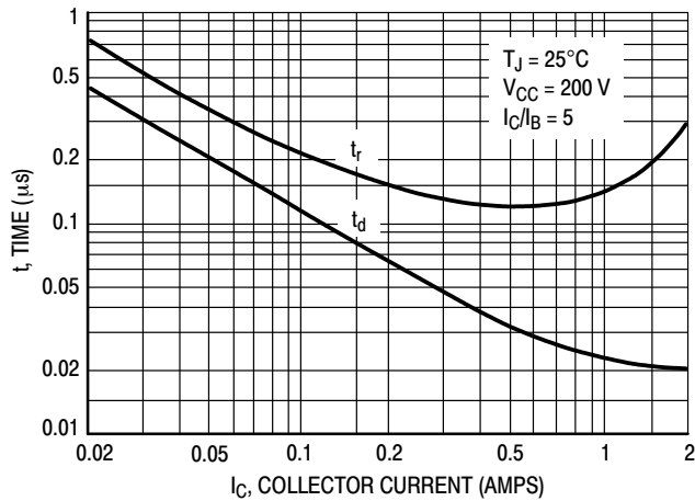
Figure 7. Turn-On Time
