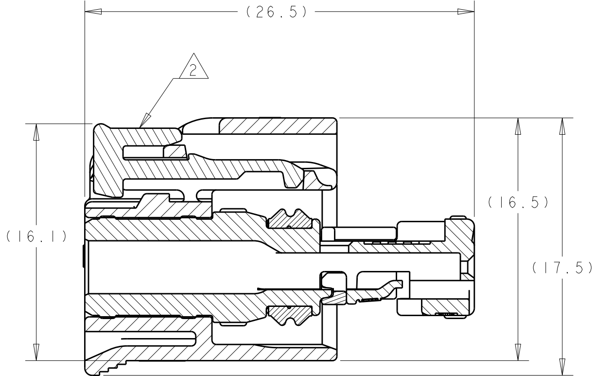
SECTION B-B
