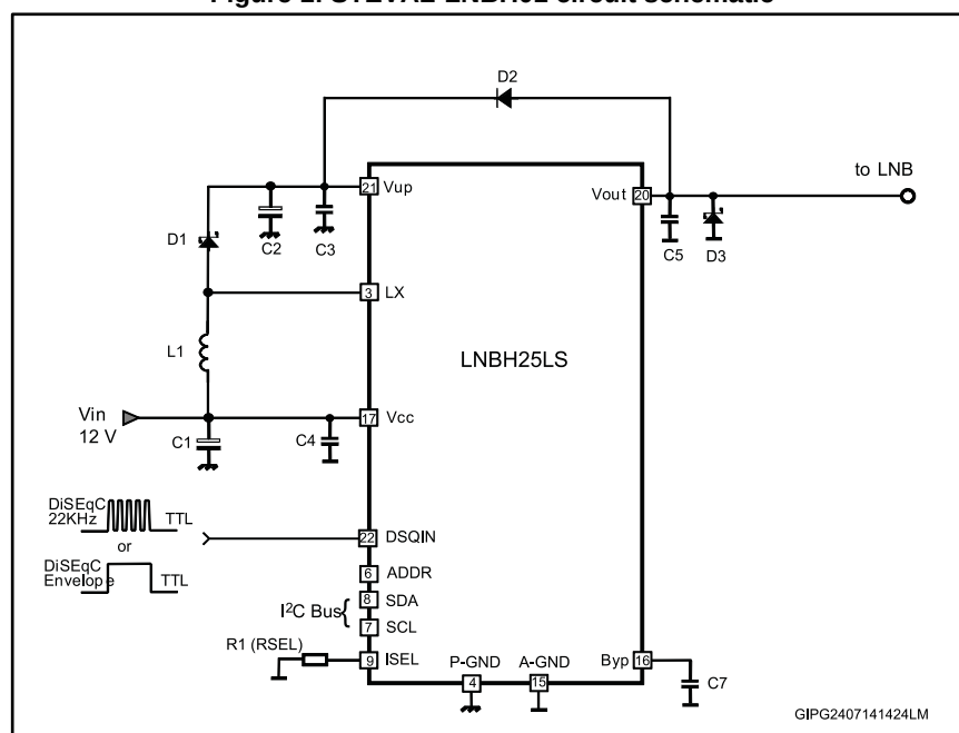
Figure 1: STEVAL-LNBH01 circuit schematic
