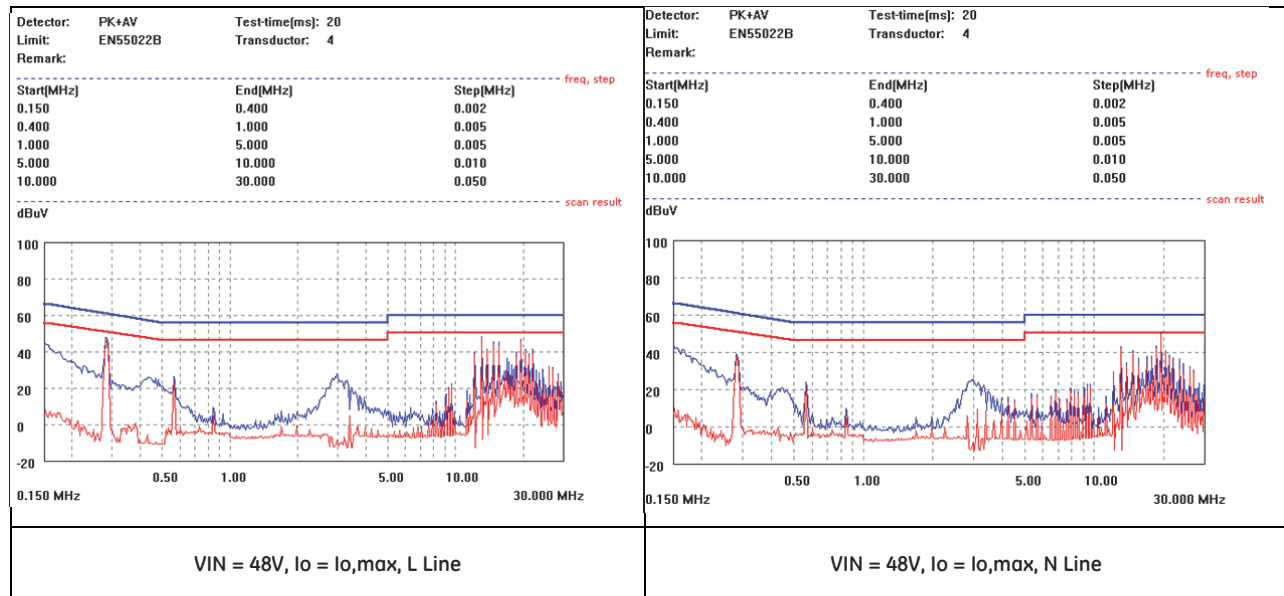
Figure 24. EMC Considerations
