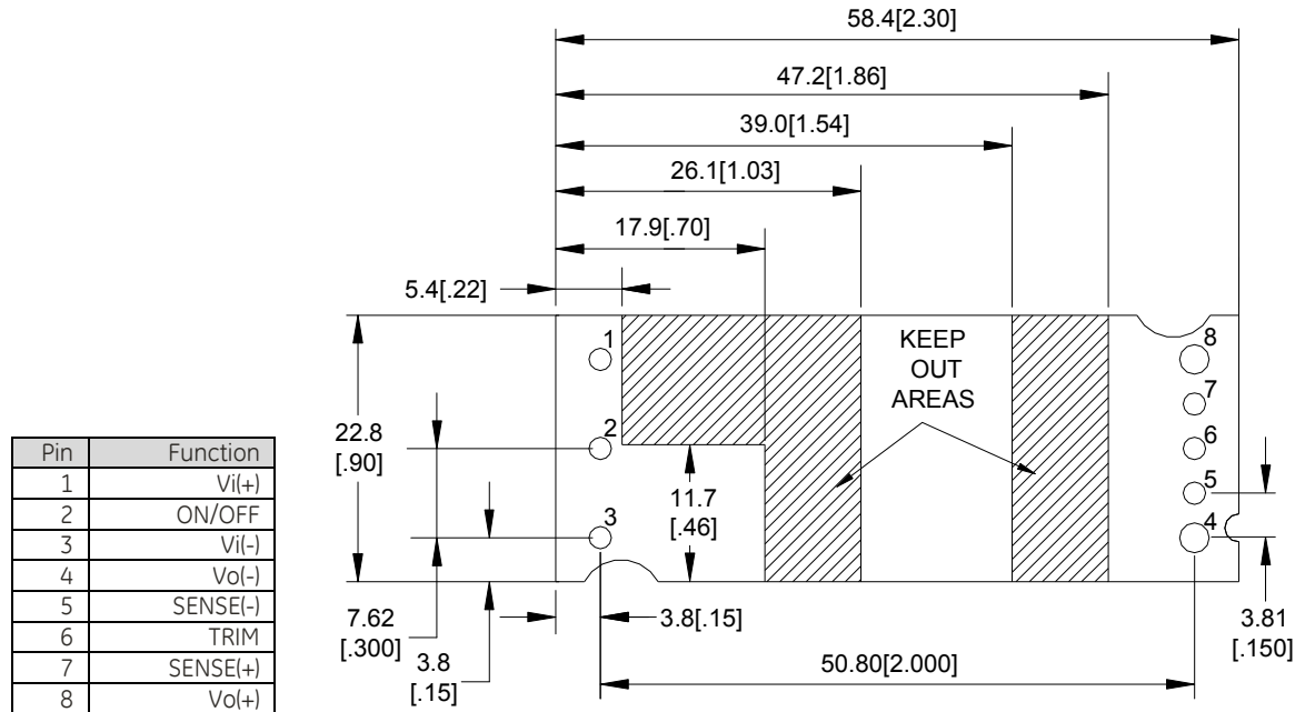
SMT Recommended Pad Layout (Component Side View)
