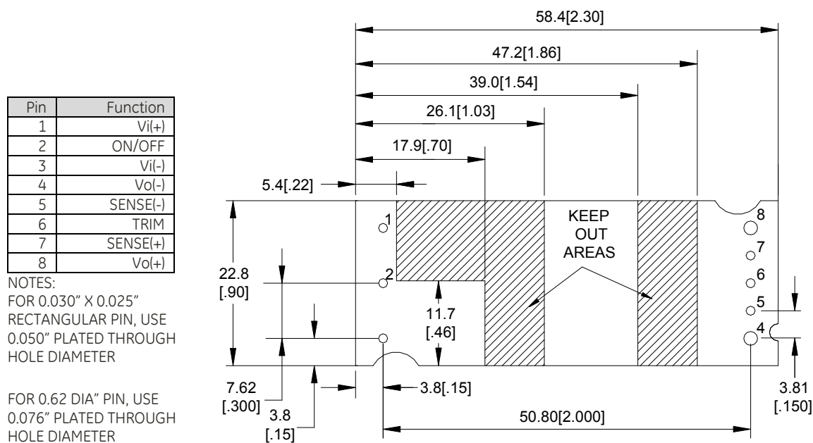
TH Recommended Pad Layout (Component Side View)
