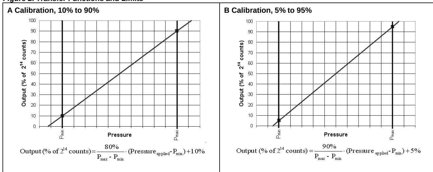
Figure 2. Transfer Functions and Limits
