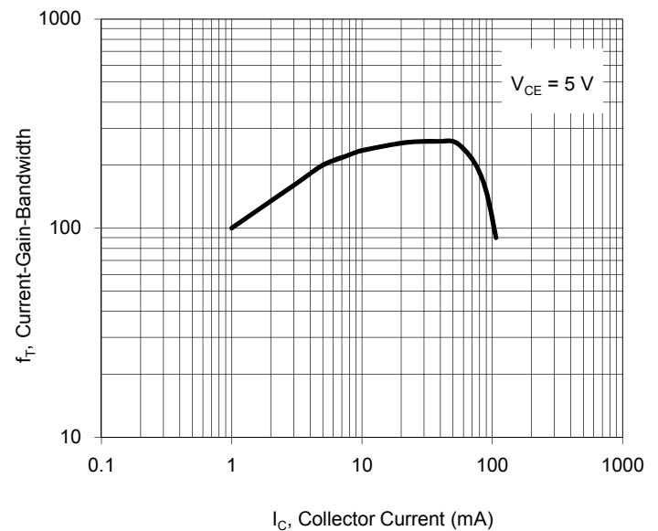
Fig.12 Current-Gain-Bandwidth Product
