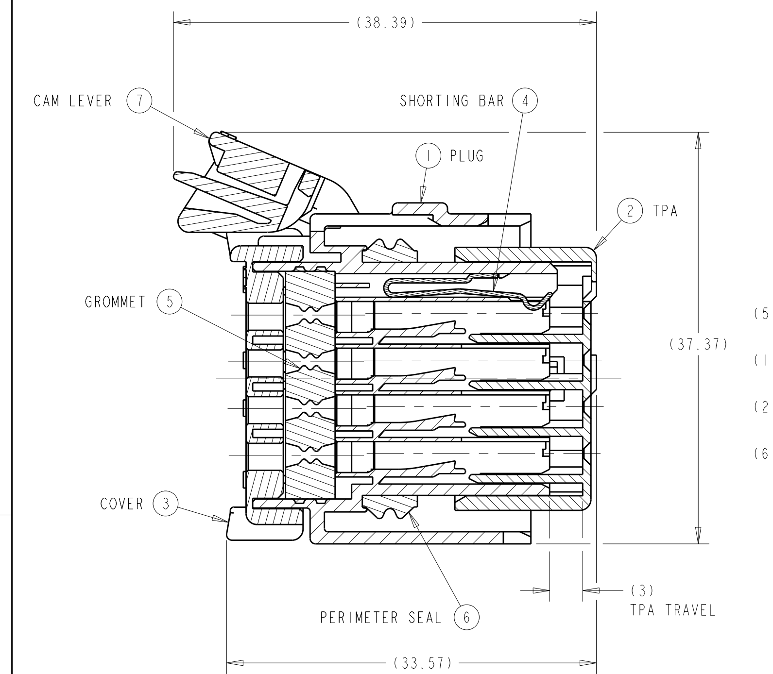
SECTION A-A SHOWN WITH CAM LEVER AND TPA IN THEIR PRE-LOADED POSITIONS (DELIVERY CONDITION)
