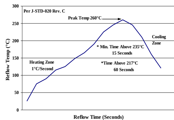
Figure 25. Recommended linear reflow profile using Sn/Ag/Cu solder.
