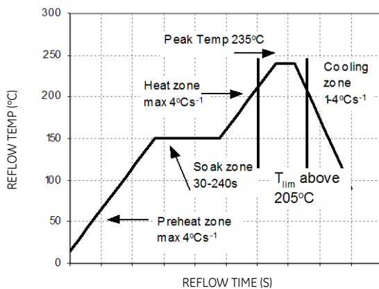
Figure 23. Reflow Profile for Tin/Lead (Sn/Pb) process.
