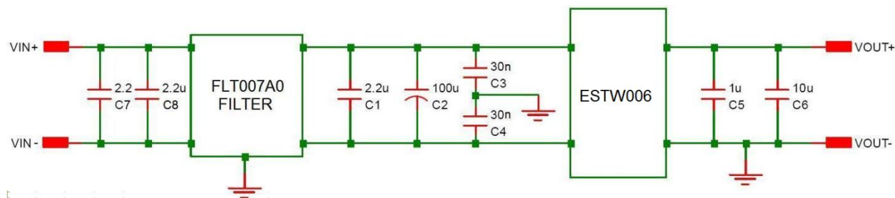
Figure 26. EMC Considerations.
