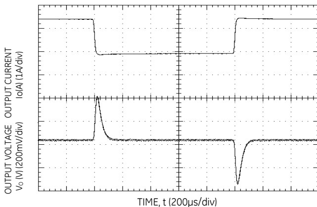
Figure 5. Transient Response to 0.1A/μs Dynamic Load Change from 50% to 75% to 50% of full load, V_{IN}=48V , C_o > 100\mu F .
