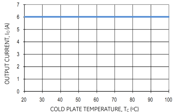
Figure 20. Derated Output Current versus Cold Wall Temperature with Local Ambient Temperature Around Module at 85°C; V_{IN} = 48 .
