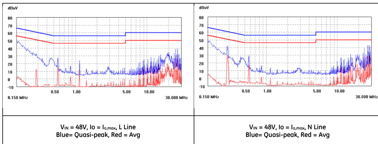
Figure 26. EMC Considerations.
