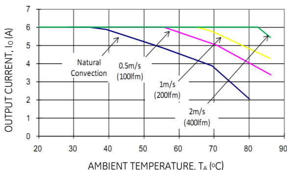
Figure 16. Output Current Derating for the Module with Heat plate; Airflow in the Transverse Direction from V_{out}(-) to V_{out}(+) ; V_{IN}=48 .
