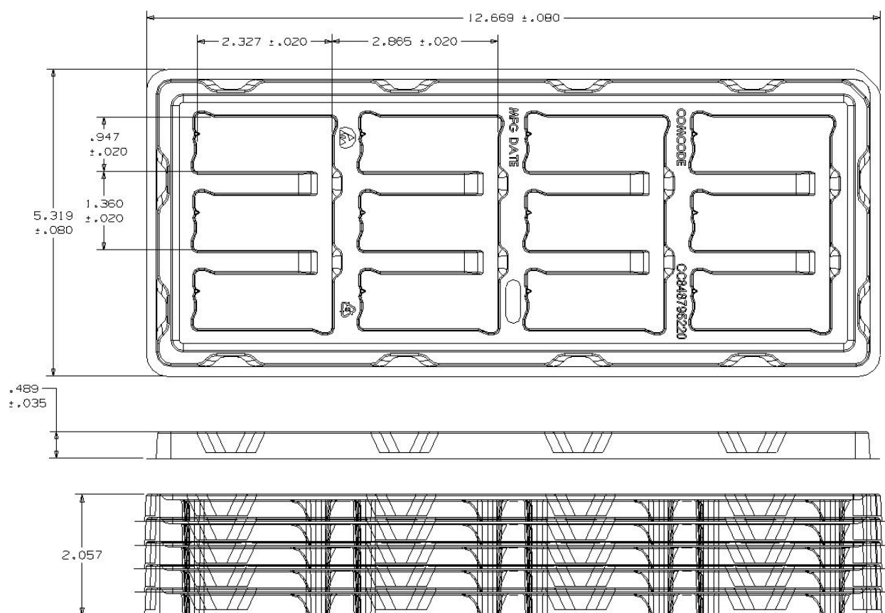
Figure 27. Surface Mount Packaging Tray.
