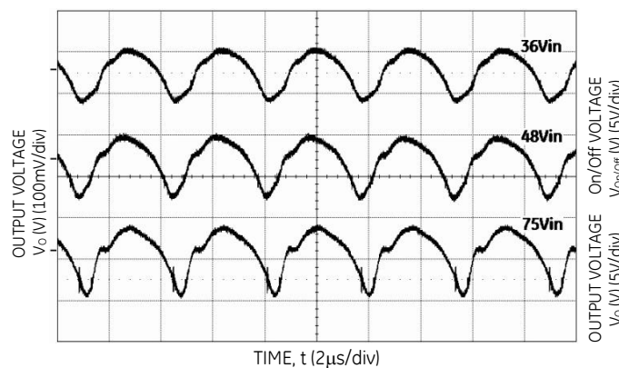
Figure 3. Typical output ripple and noise ( I_o = I_{o,max} ).
