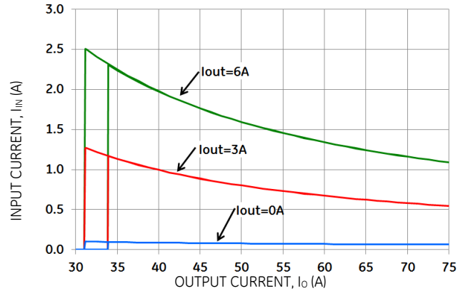
Figure 2. Input Current versus Output Current.
