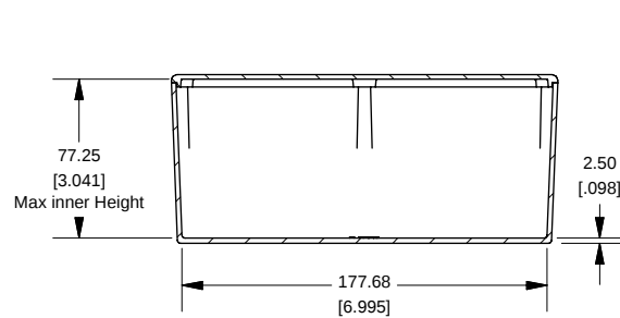
SECTION B-B Side View of Assembly
