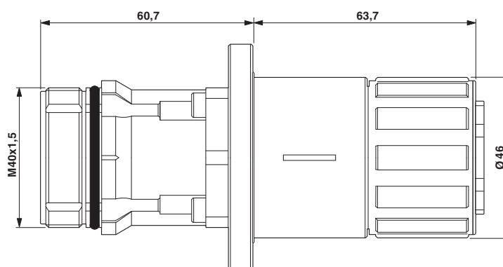
Dimensional drawing
