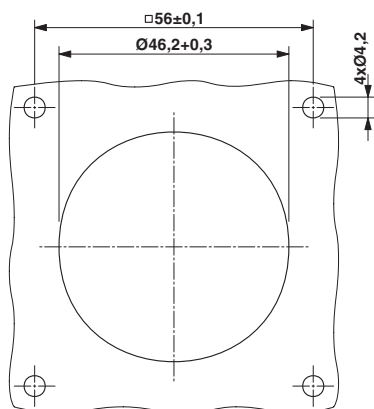
Dimensional drawing
