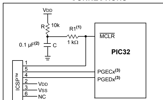
FIGURE 2-2: EXAMPLE OF MCLR PIN CONNECTIONS (1,2,3)
