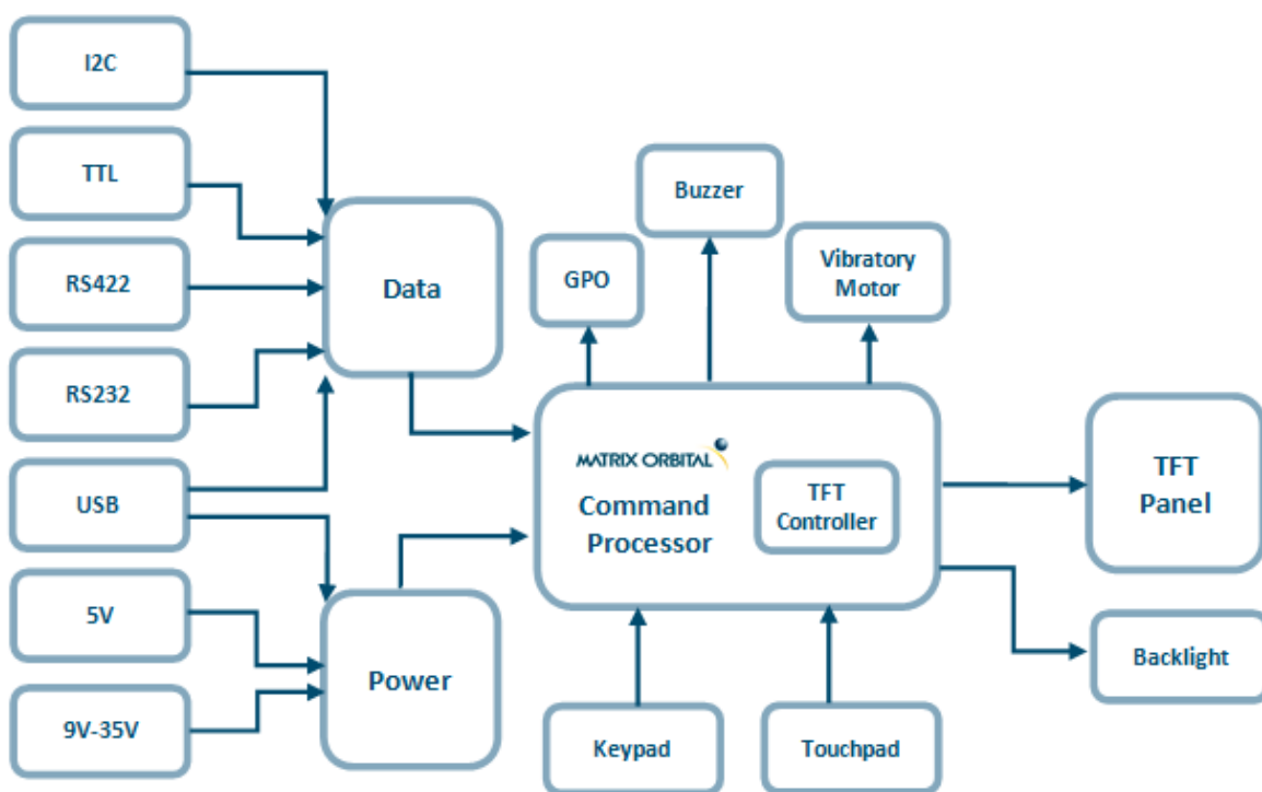
Figure 2: Functional Diagram
