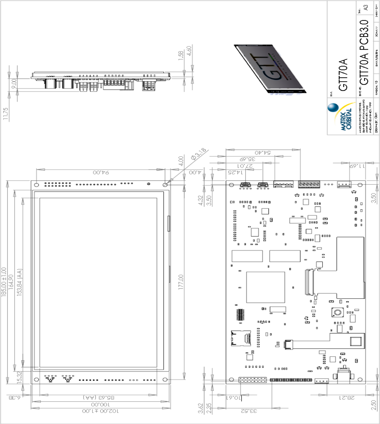
Figure 18: GTT70A Drawing
