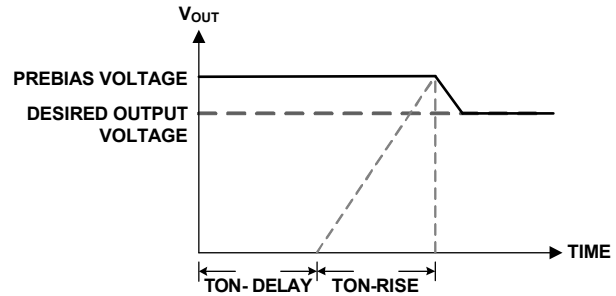
FIGURE 28. OUTPUT RESPONSES TO PREBIAS VOLTAGES
