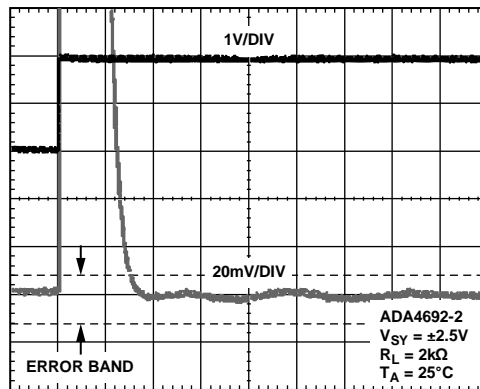
Figure 54. Positive Settling Time to 0.1%
