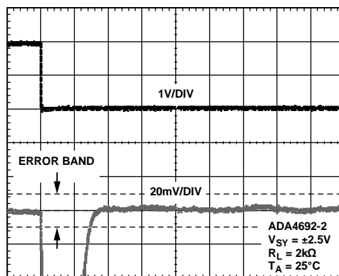
Figure 55. Negative Settling Time to 0.1%
