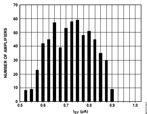
Figure 8. Supply Current Distribution, V_S = 5\text{ V}
