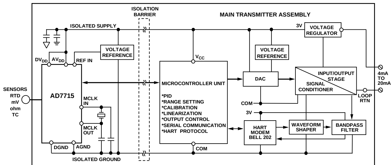
Figure 17. Smart Transmitter Using the AD7715
