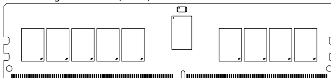
Figure 1: 288-Pin RDIMM (MO-309, R/C-E1, E2)
